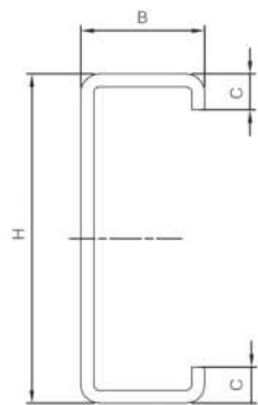
C型檩条规格 Sizes of C-shape purlins
